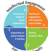
Figure 1. AST practices
